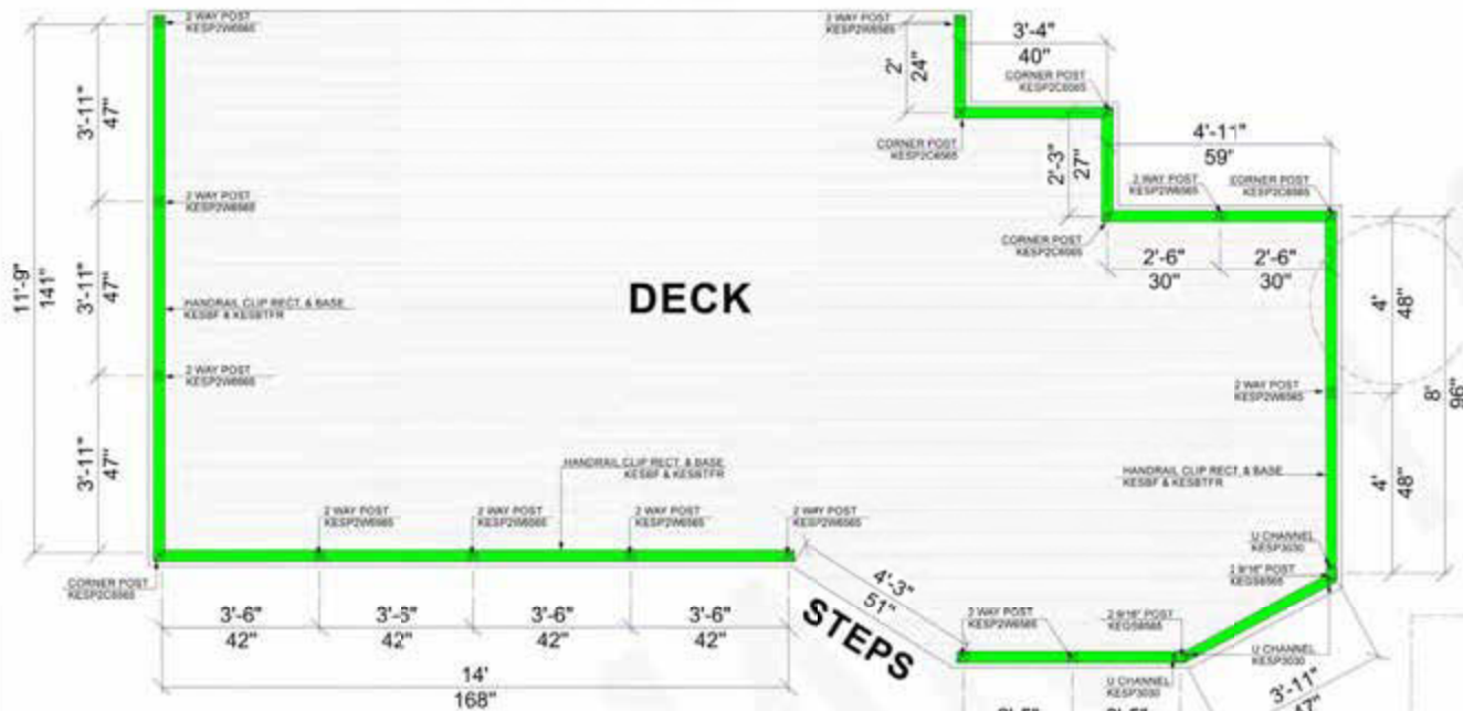
RAILING FLOORPLAN
