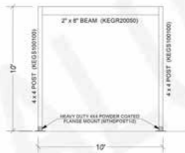
PERGOLA DETAIL SIDE ELEVATION
